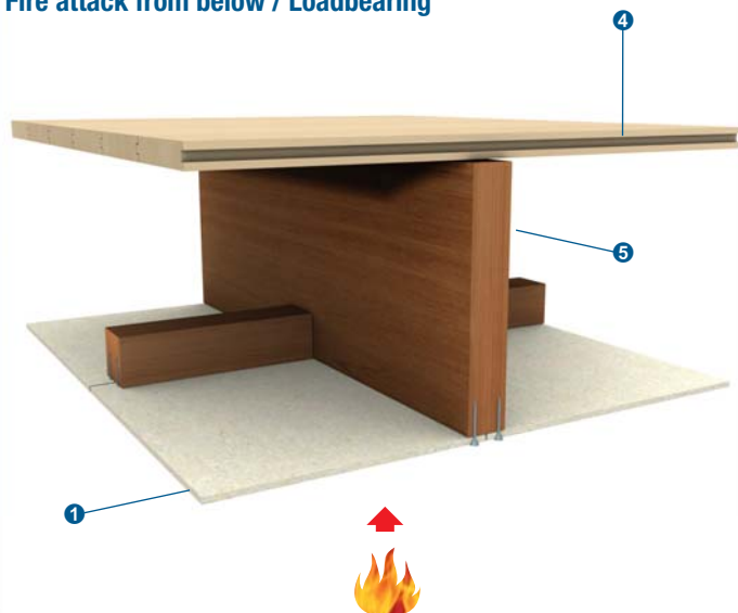
Fire attack from below / Loadbearing
