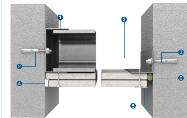
Self-supporting ceiling perimeter to wall intersection (case 2)
