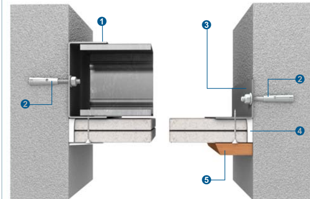
Self-supporting ceiling perimeter to wall intersection (case 1)
