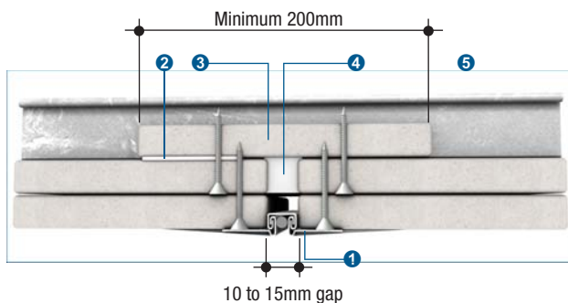
Perpendicular to steel framing of double layer self-supporting ceilings
